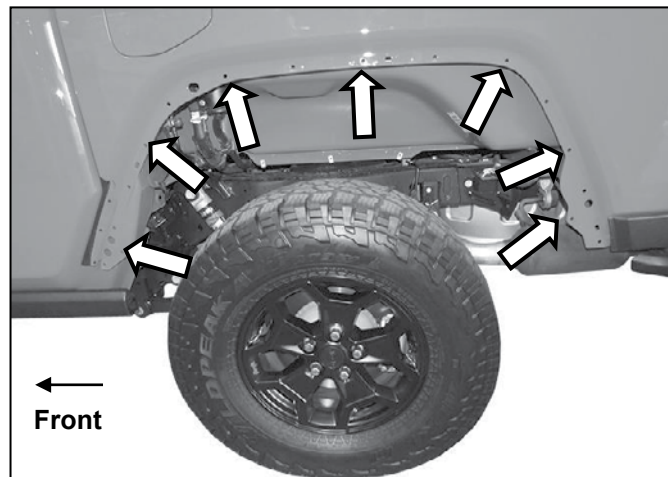
(Fig 5) Do not drill these (7) mounting locations. NOTE: The (7) mounting locations can be accessed from between body panels
