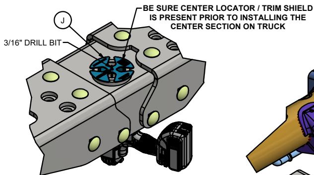
PILOT HOLE DRILL GUIDE
