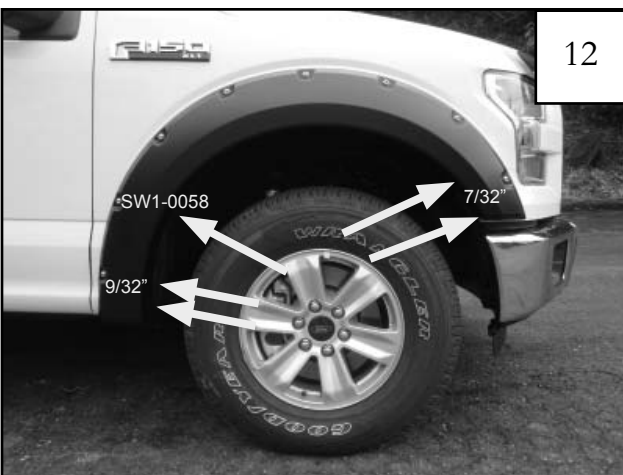
Still holding flare to fender, re-install remaining factory screws removed in Step 4 using 7/32" and 9/32" sockets and wrench. Using a phillips screwdriver, install supplied screw (SW1-0058) into Clip (CL1-0009). Tighten all screws.
