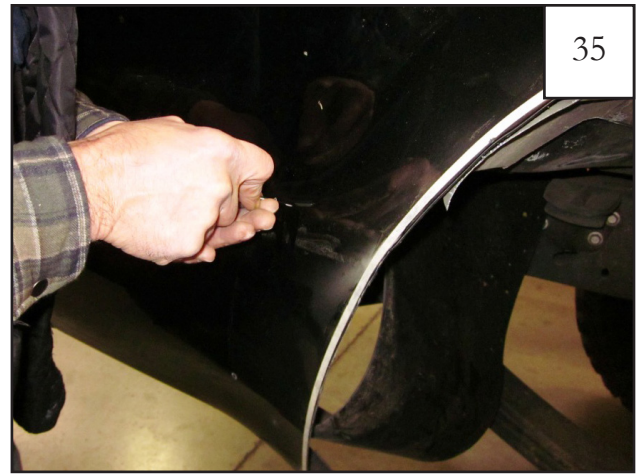
Remove flare. Using marks made with scratch awl as a guide, score the sheet metal with a center punch prior to drilling.
