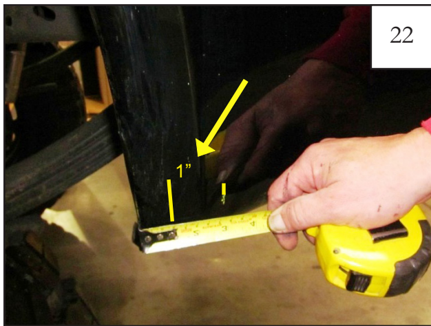
Measure 1" from back side of rear wheel well and front wheel well and mark using a grease pencil.
