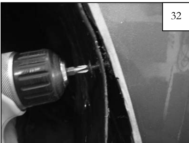
32 Starting with the top location, fasten inner fender metal to bent tabs of outer fender with Screw (SW1-0056)s through holes drilled in last step (3 locations).
