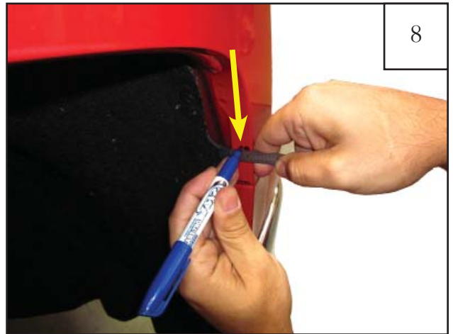
Remove the flare. At the marked locations made in Step 6, measure inward 22mm from the edge of the fender and mark with grease pencil or marker. These are the marks to be drilled.
