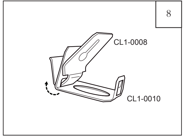
8 Assemble Clip CL1-0008 with CL1-0010 as indicated in the above diagram. Insert tab of CL1-0008 through slot in CL1-0010.
