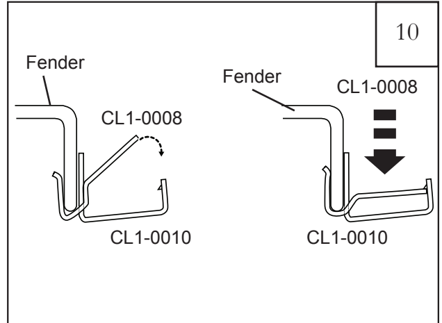
10 Press down on CL1-0008 as indicated until an audible “snap” is heard. NOTE: This may require pliers.
