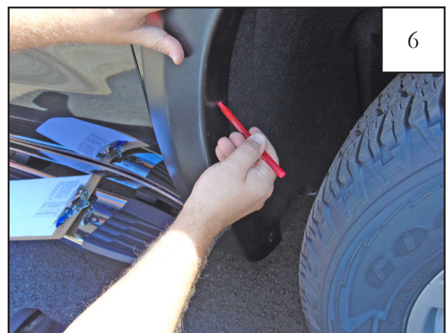
Use a grease pencil to mark the two locations of the holes indicated with the circles in Step 5. Remove flare from vehicle.
