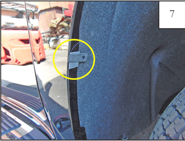
7 Install supplied Tab (MT1-0034) over the rear location marked in Step 6. Install a Clip (CL1-0009) as indicated on top of the protective film.
