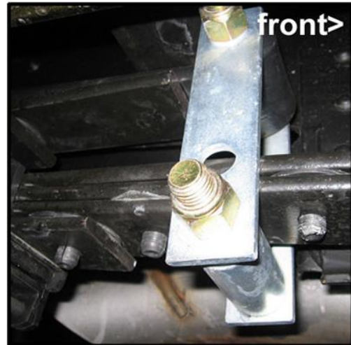
adjustable pre-load & ride height
