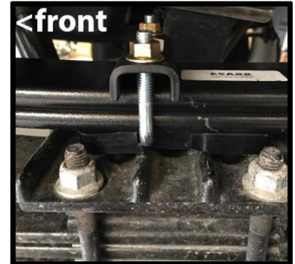
Install the SuperSprings as pictured below, then thread the channel crossplate on to the ubolt. Tighten securely.
