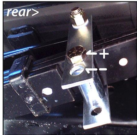
Rear Shackle installation
