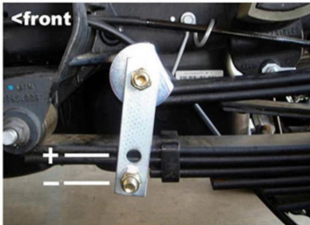
Place PSP-19 on top of spring plate flat side up facing, with groove toward the front
