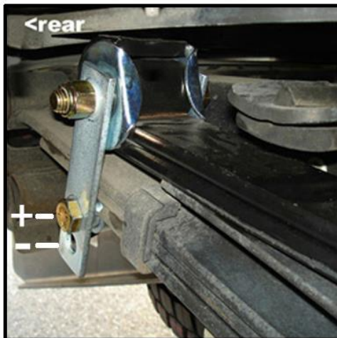
Adjustable spring pre-load & ride height
