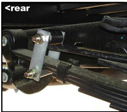
Trim shackle length ~ Use upper hole
