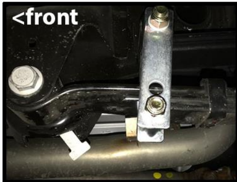
PSP-19 with hold-down clamp assembly
