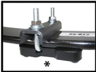
PSP-19 with hold-down clamp assembly
