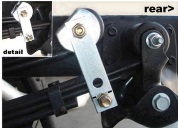
Place PSP-19 on top of spring plate flat side up facing, with groove toward the front
