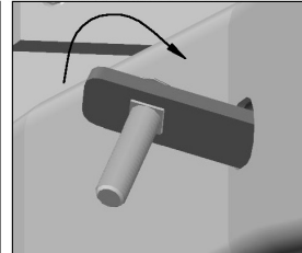
ROTATE THE LOCKING STRAP CLOCKWISE UNTIL IT HITS THE BOTTOM OF THE TRUCK FRAME
