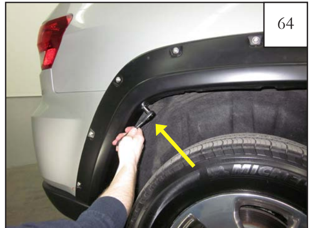
64 While holding Flare on vehicle, install factory fasteners removed in Step 31 & Step 57 using a 10mm socket and wrench. Do not fully tighten at this time.
