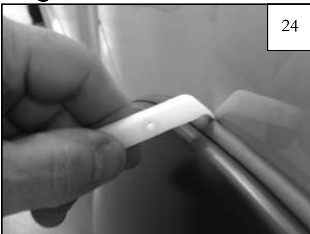
24 Using supplied Edge Trim Tool (ET1-0002), seat edge trim against vehicle by hooking curved end under edge trim at one end of flare. Next, slide around outer edge of flare to the other end.
