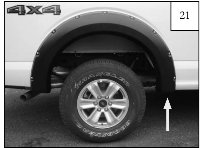
21 Start a supplied screw (SW1-0050) through the flare into the clip installed in Step 19. Tighten all screws.
