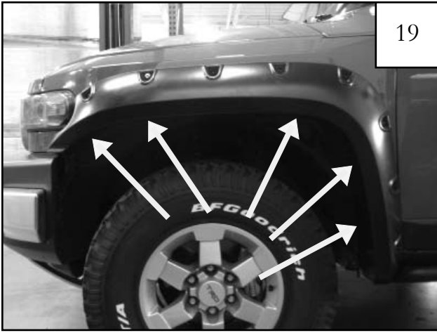
Position Flare on fender. Install five supplied Screws (SW1-0036). Do not tighten. NOTE: It is helpful to install one of the top bolts first.
