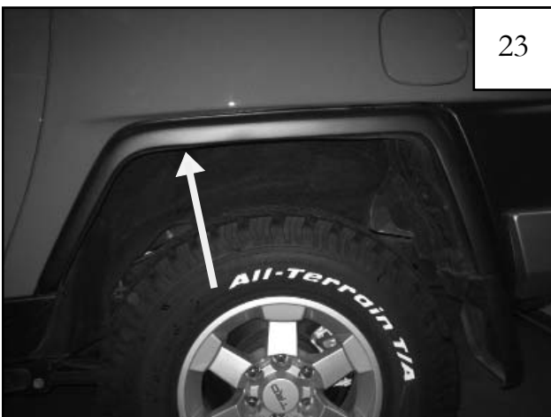
Using a pry tool or flat head screwdriver, remove one plastic fastener.
