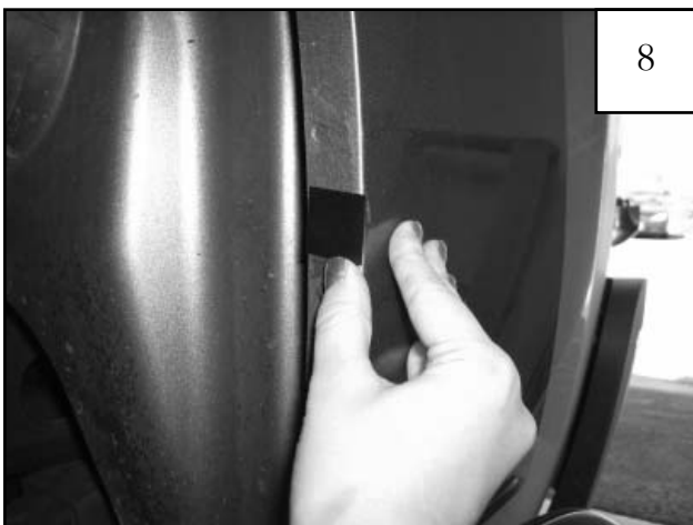
Center a supplied Black Plastic Tab over the remaining four marks made in Step 4, aligning edge of tab with inside of fender lip (tab may extend over outside of fender).
