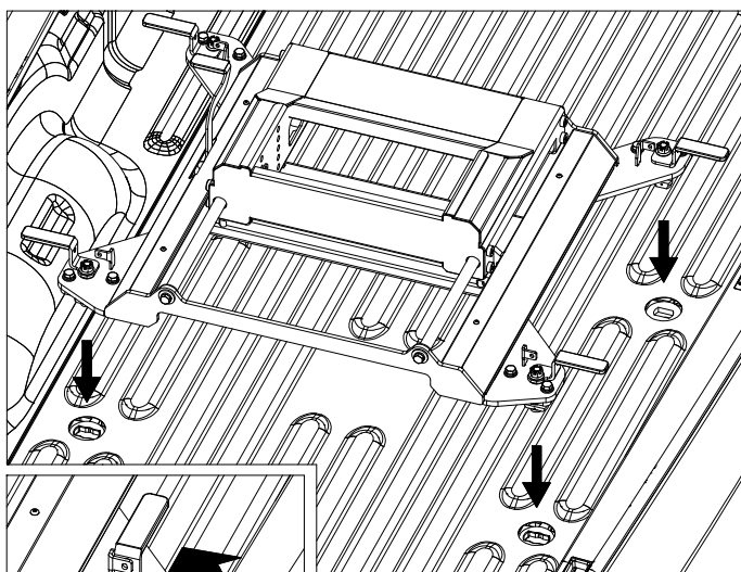
Figure B1: View of unlatched base.
