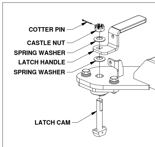
Figure B5: List of latch parts.
